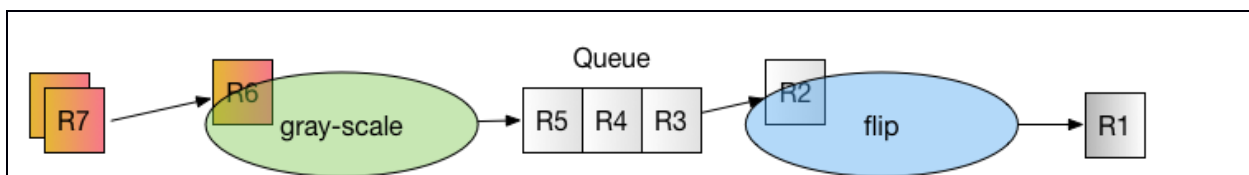
Figure 11: Implementing a pipeline with a queue.
