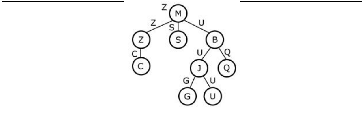
Figure 15: Search tree.
