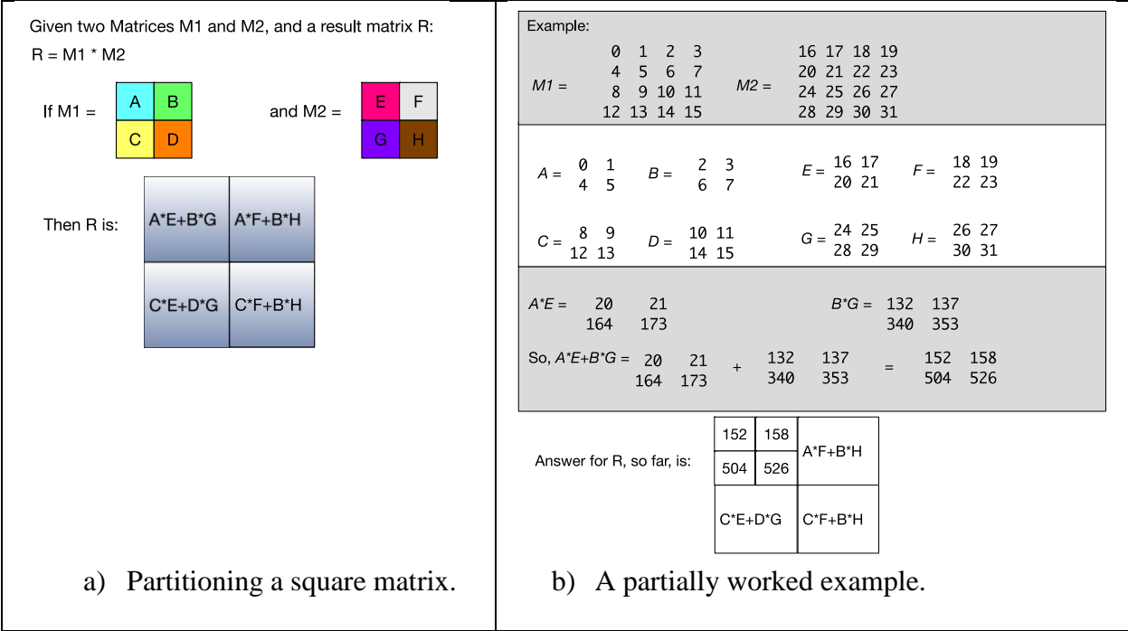
Figure 9: First step of recursive Matrix Multiply
